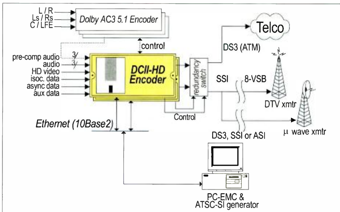
Figure 1. For HD applications, the DCII-HD encoder feeds either an ATM telco network or a microwave STL with DS-3 input.
