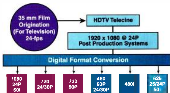
Figure 10 The 24-frame progressive HDCAM system provides a “super-sampled” HD master that downconverts with very high quality to multiple distribution formats for DTV broadcasting.
