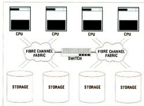
Figure 2. Fibre channel architecture can employ loop or fabric topology and can be switched.
