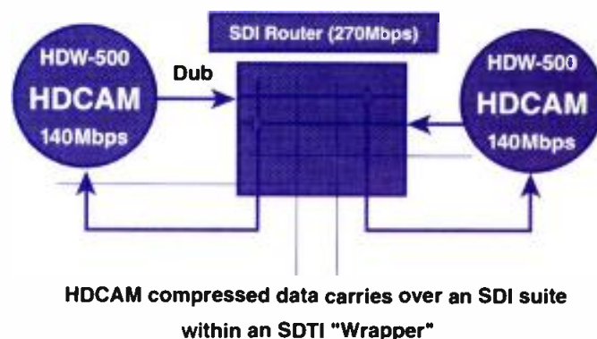
Figure 7 The 140Mbits/s digital dub video is mapped within an SDTI protocol to provide a convenient means of routing the HD signal within a standard 270Mbits/s system.
